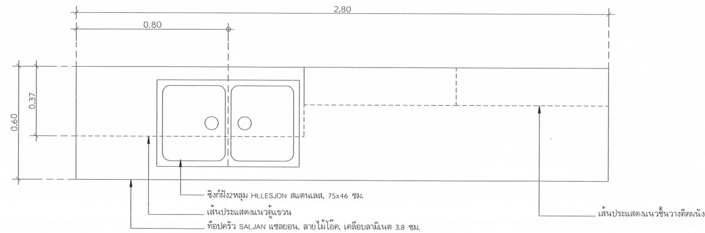
TOP VIEW B-10 Kitchen Cabinet L280xW60xH92 cm. (IKEA) SCALE 1:20 OPTION 1
