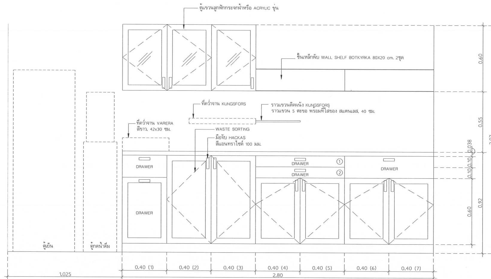
FRONT VIEW B-10 Kitchen Cabinet L240xW60xH80 cm. (IKEA) SCALE 1:20
