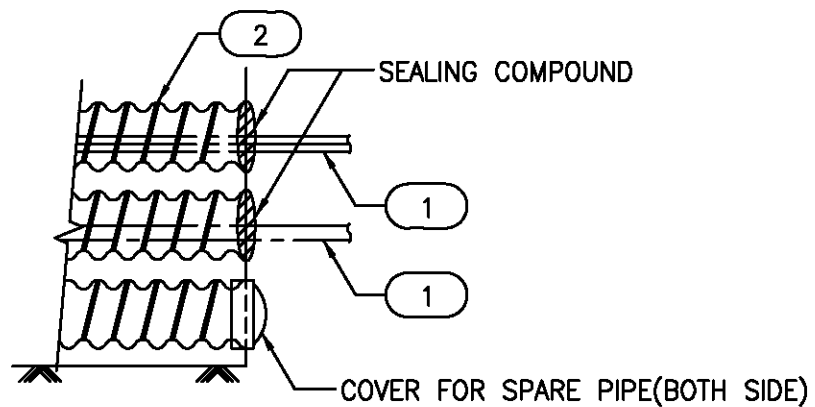
DETAIL "B"
